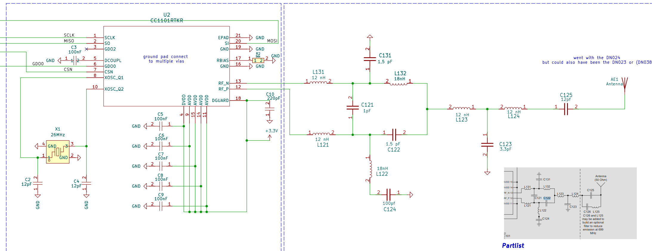
Texas Instruments Balun And Impedance matching
